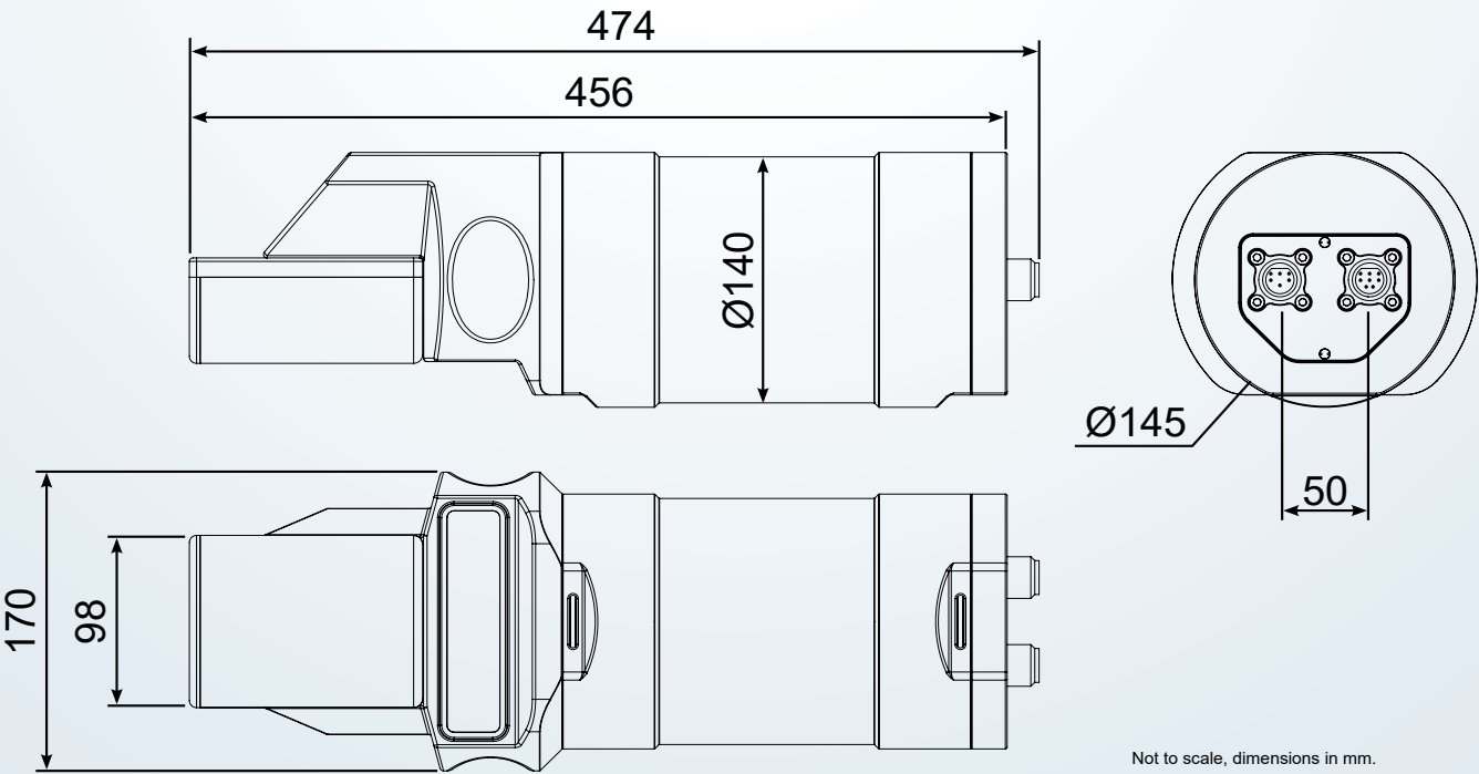
Not to scale, dimensions in mm.
